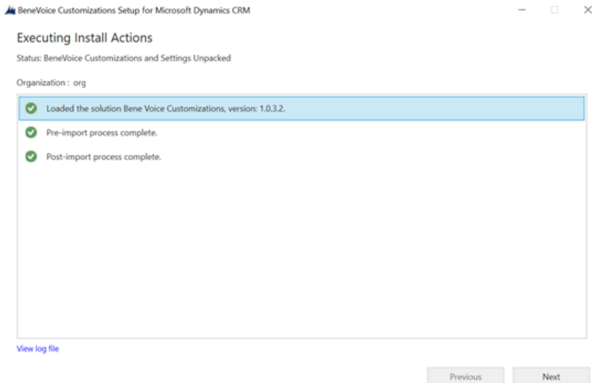
Figure 19 Installer Configuration
