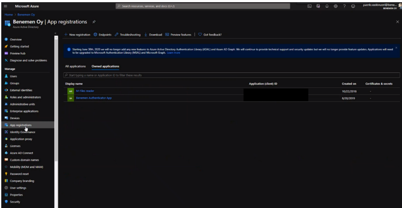
Figure 5 App registrations
