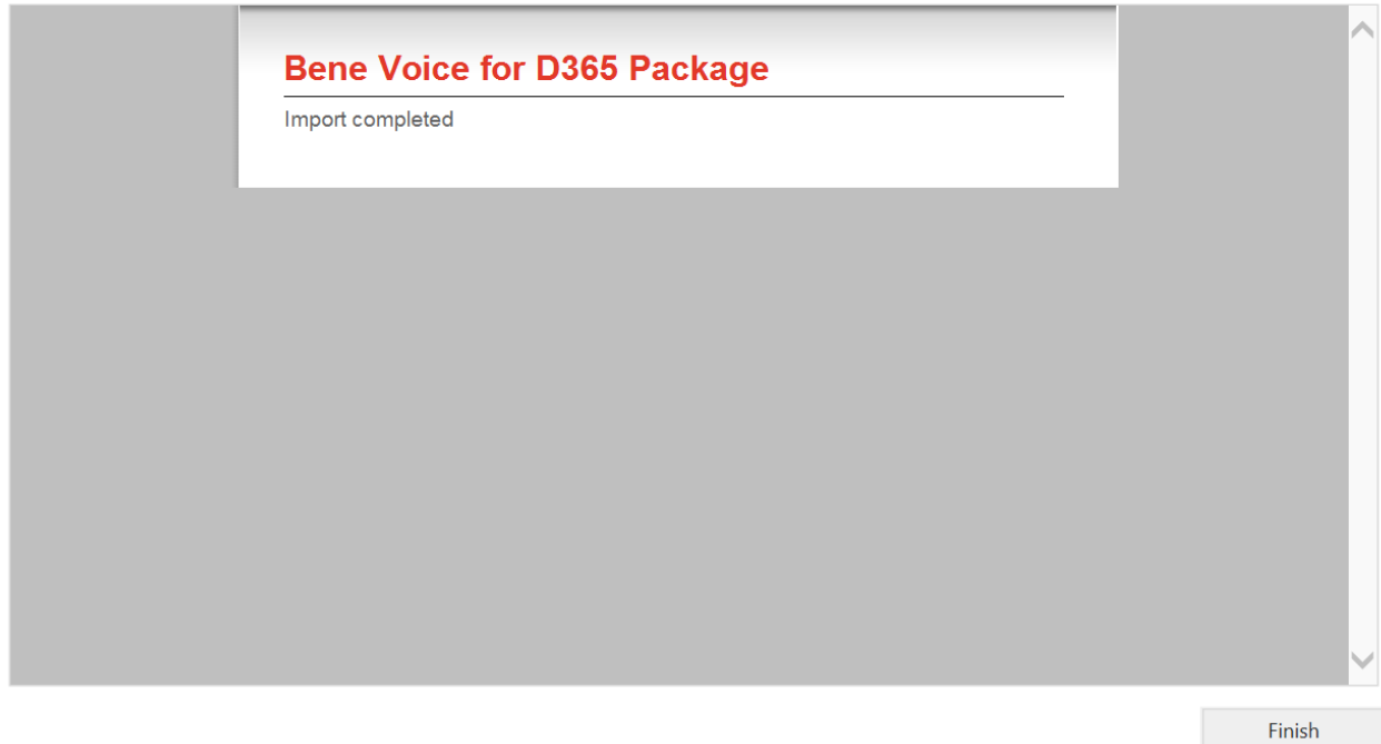
Figure 21 Installation Complete
